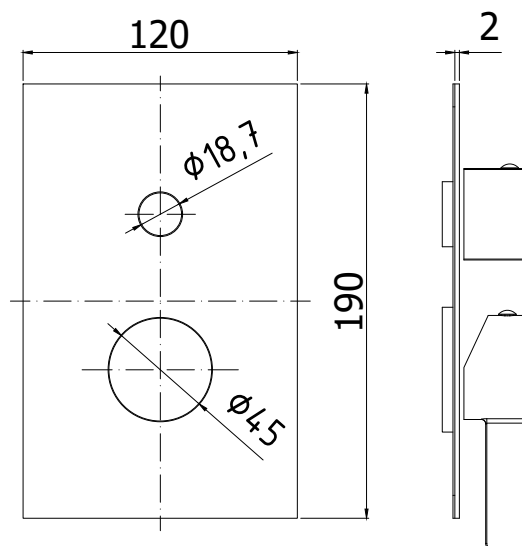
TECHNICAL DRAWING
